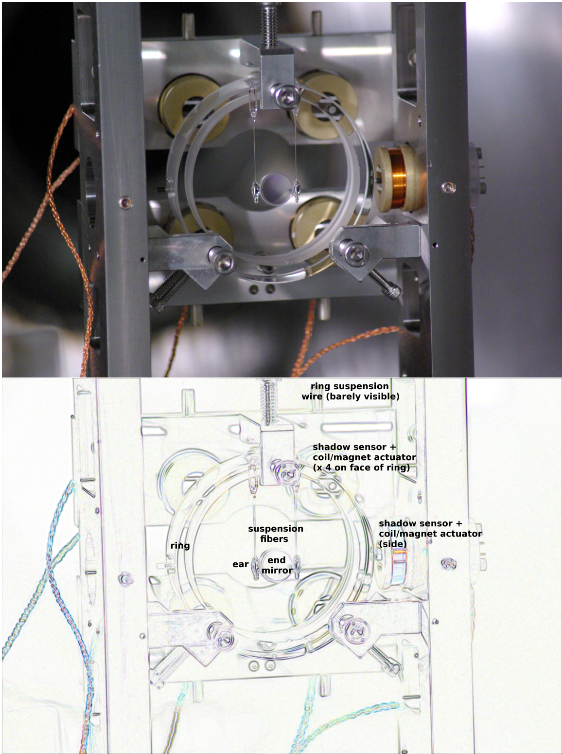
Figure 3-3: The 1 gram end mirror and its suspension.
