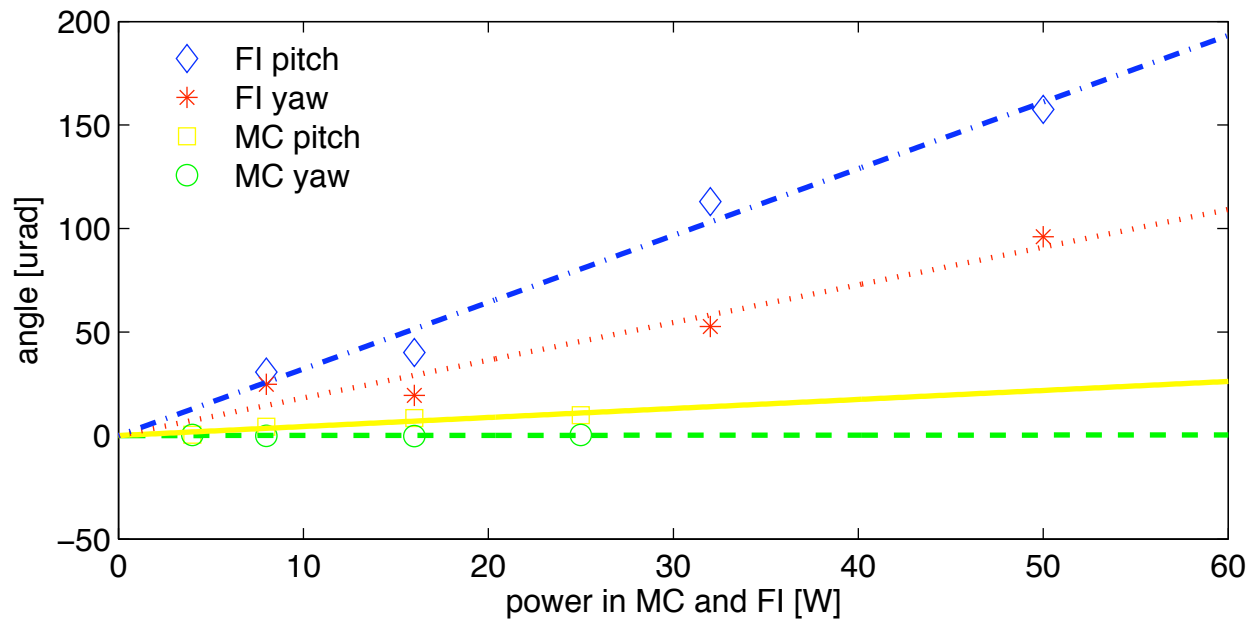
Figure 3-10. Mode cleaner and Faraday isolator thermal drift data. A) Angular motion of the beam at the MC waist and FI rotator as the input power is stepped. The beam is double-passed through the Faraday isolator, so it experiences twice the input power. B) Average beam angle per power level in the MC and FI. Linear fits to the data are also shown. The slopes for MC yaw, MC pitch, FI yaw, and FI pitch, respectively, are 0.0047, 0.44, 1.8, and 3.2 \mu\text{rad}/\text{W} .
