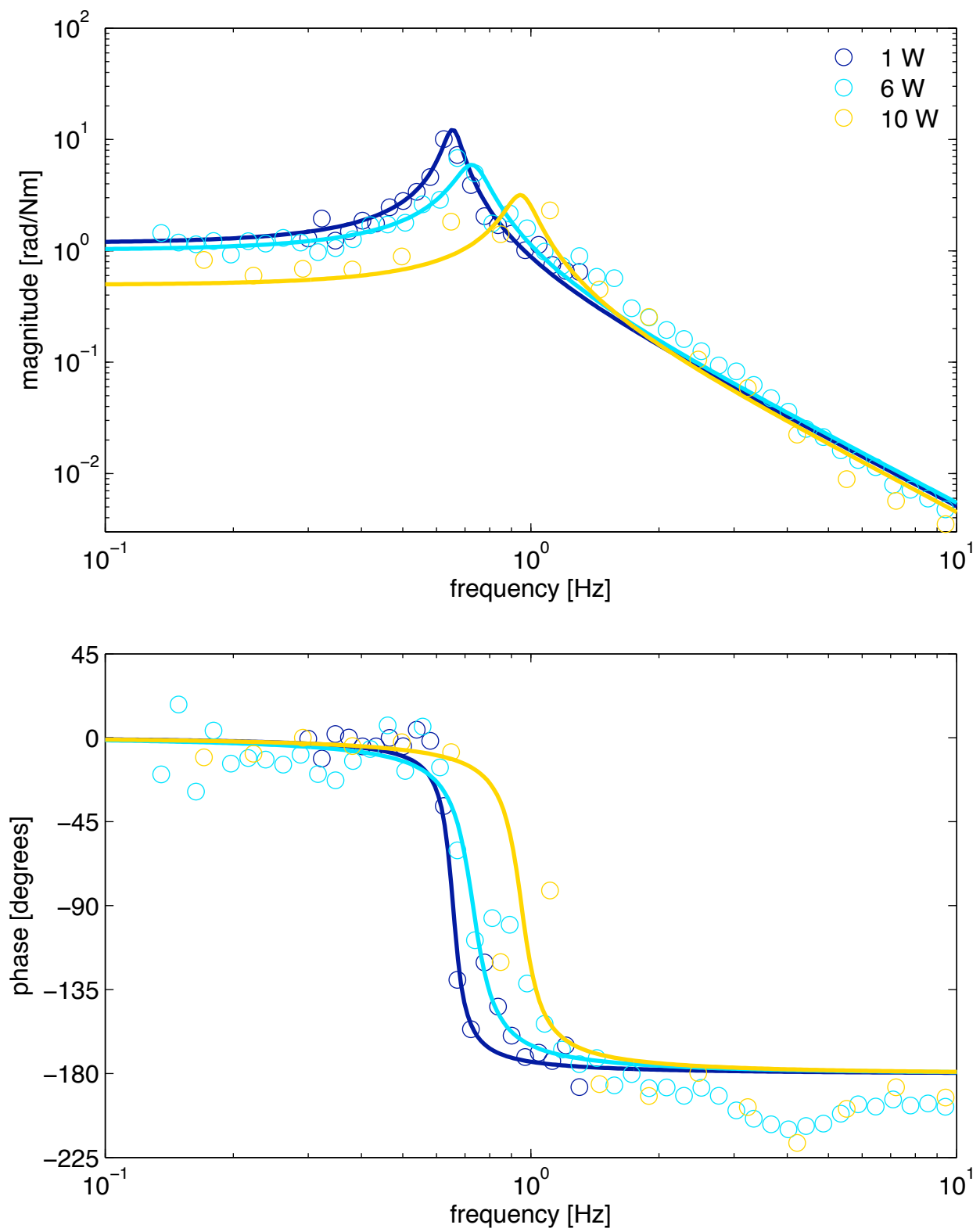
Figure 6-17. Hard opto-mechanical mode measurement and fit for several powers.
